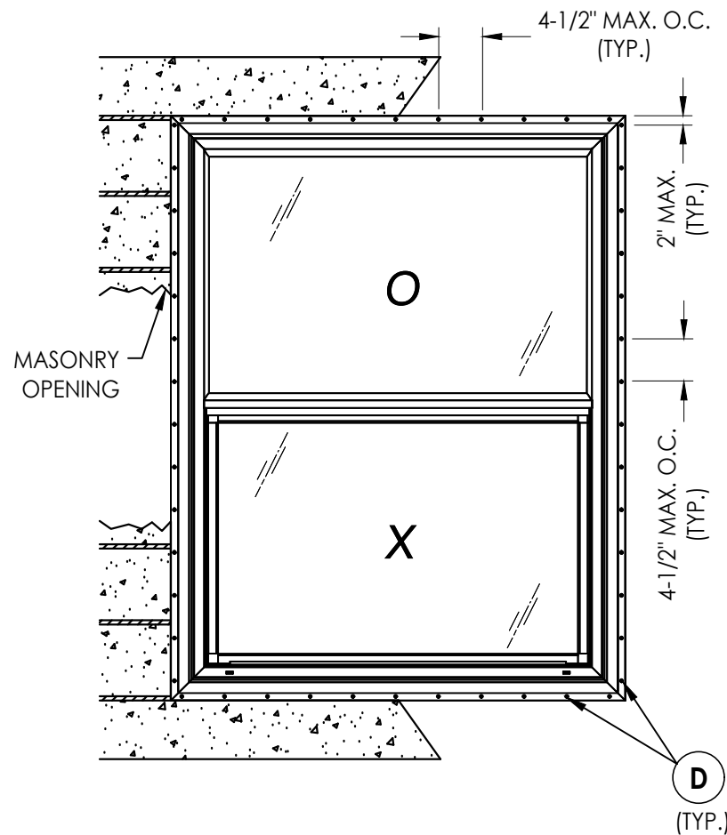
FRAME ANCHORING MASONRY CONSTRUCTION
