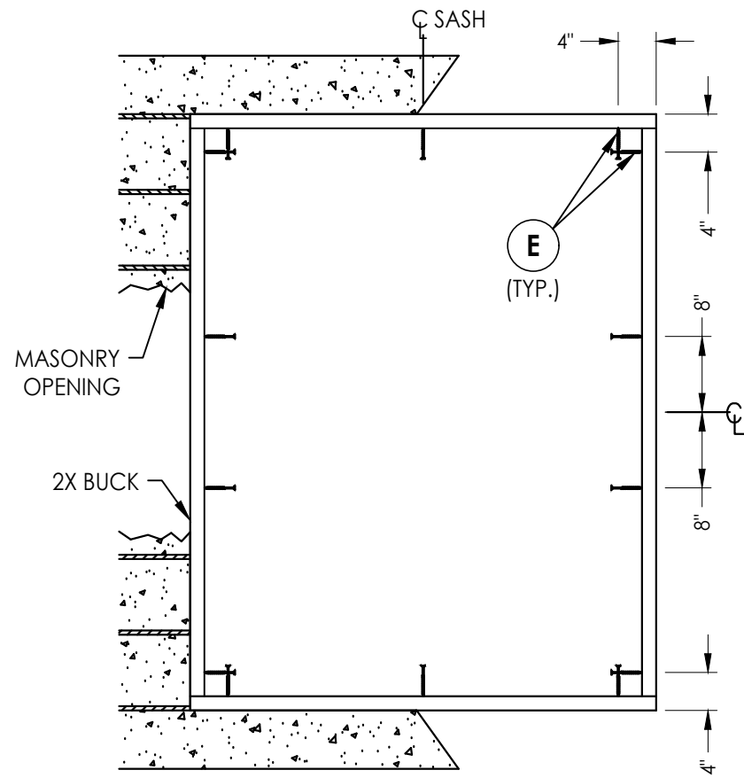
BUCK ANCHORING
